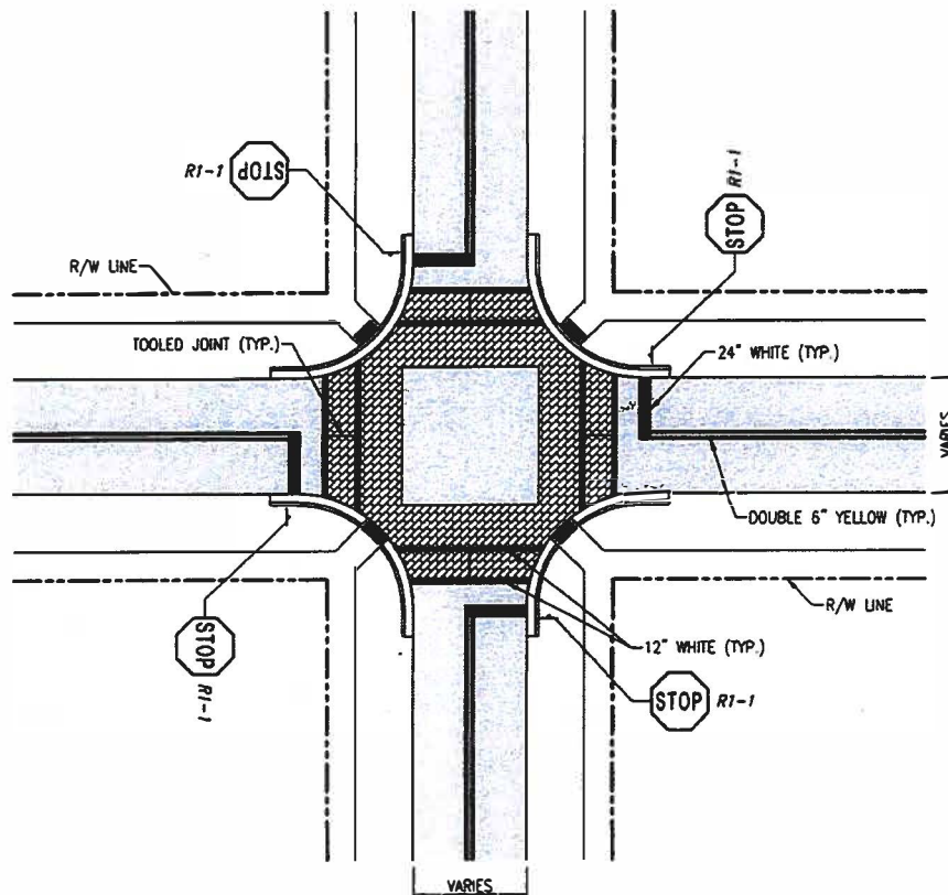
RAISED INTERSECTION DETAIL SCALE: 1"=20'
